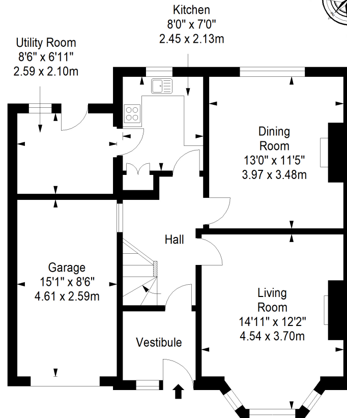
Ground Floor Approx. 65.6 sq. metres (706.1 sq. feet)
